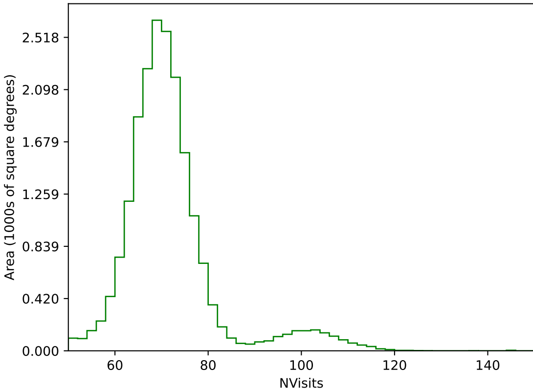
extra_ss_neo7_v3.4_10yrs All sky g band: NVisits
