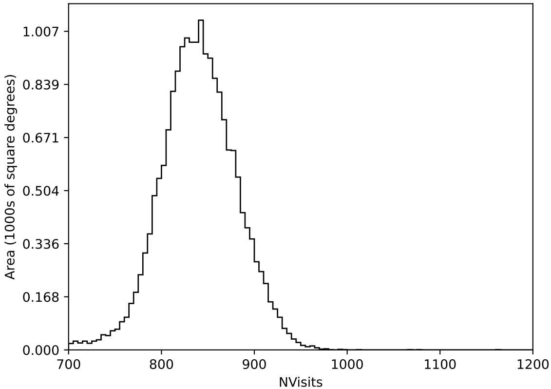
extra_ss_neo7_v3.4_10yrs All sky all bands: NVisits
