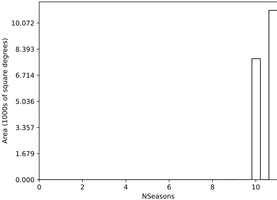
extra_ss_neo7_v3.4_10yrs WFD all bands: NSeasons
