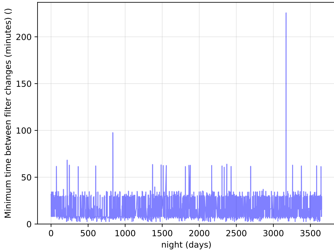
extra_ss_neo7_v3.4_10yrs Per Night: Minimum time between filter changes (minutes)
