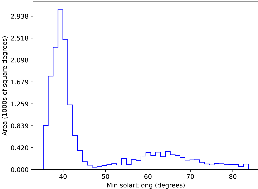
extra_ss_neo7_v3.4_10yrs WFD all bands: Min solarElong
