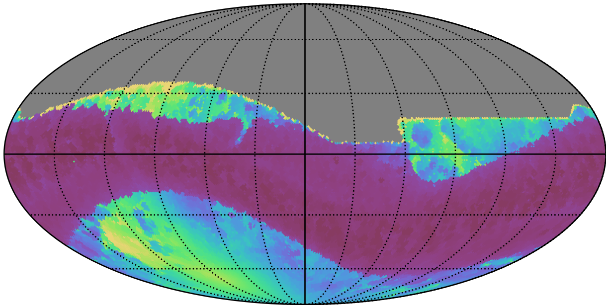
extra_ss_neo7_v3.4_10yrs All sky all bands: Min solarElong
