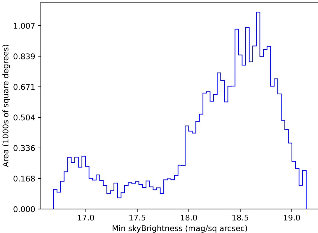
extra_ss_neo7_v3.4_10yrs Yr 1 z band: Min skyBrightness
