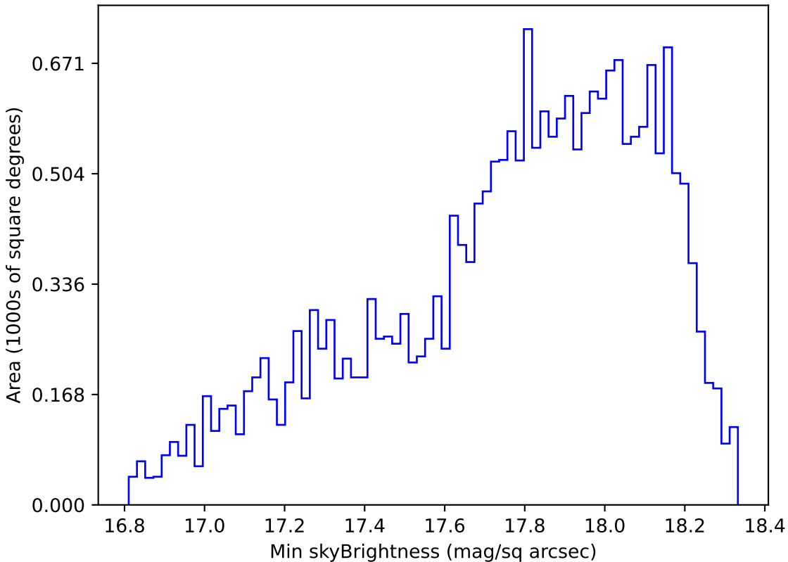
extra_ss_neo7_v3.4_10yrs Yr 1 y band: Min skyBrightness
