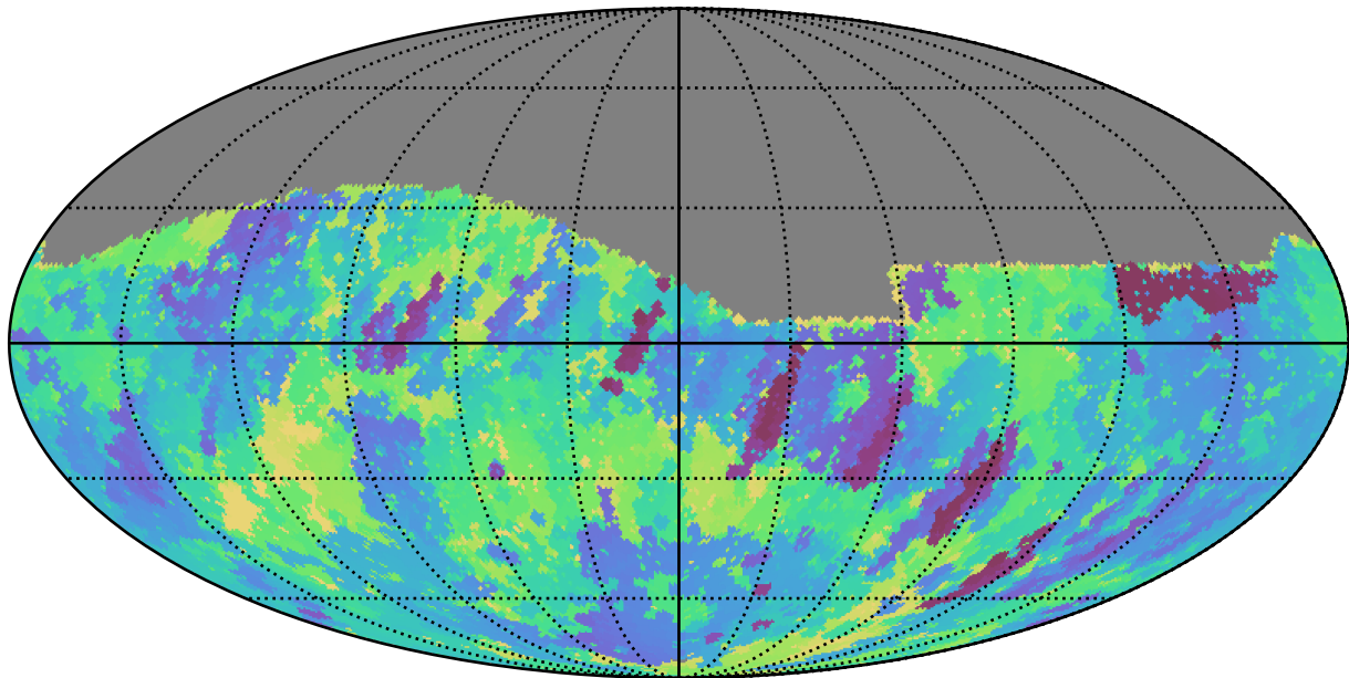
extra_ss_neo7_v3.4_10yrs Yr 1 r band: Min skyBrightness
