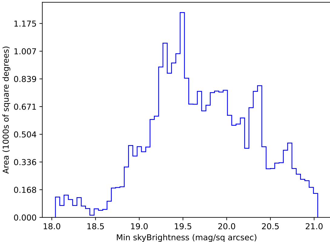
extra_ss_neo7_v3.4_10yrs Yr 1 r band: Min skyBrightness
