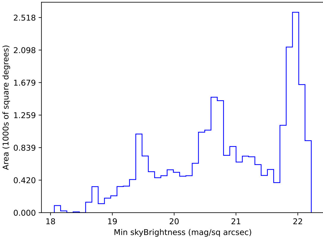
extra_ss_neo7_v3.4_10yrs Yr 1 g band: Min skyBrightness
