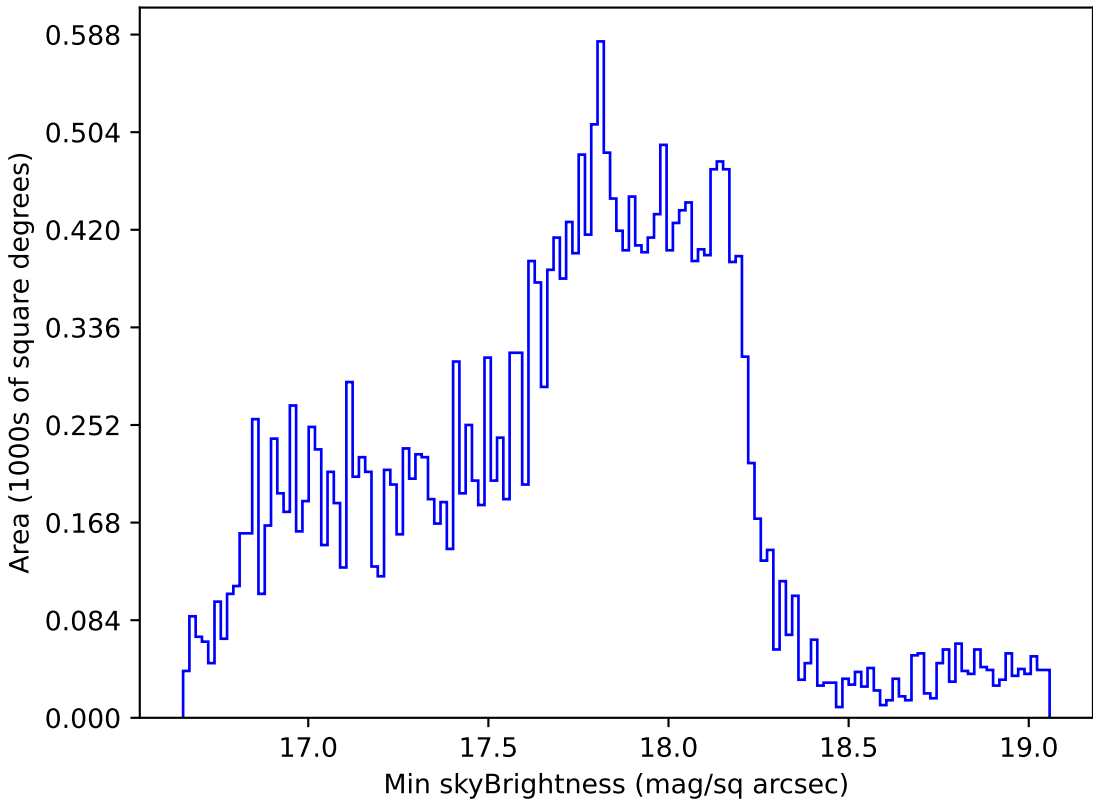
extra_ss_neo7_v3.4_10yrs Yr 1 all bands: Min skyBrightness
