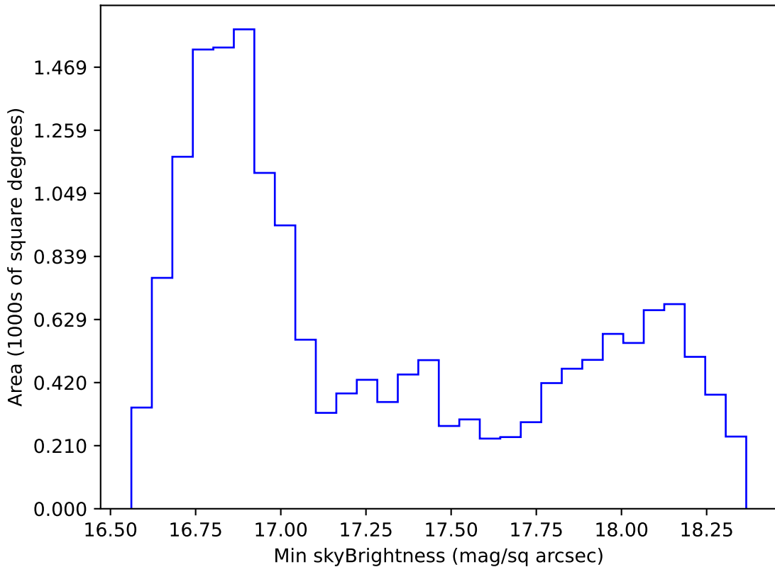
extra_ss_neo7_v3.4_10yrs WFD z band: Min skyBrightness
