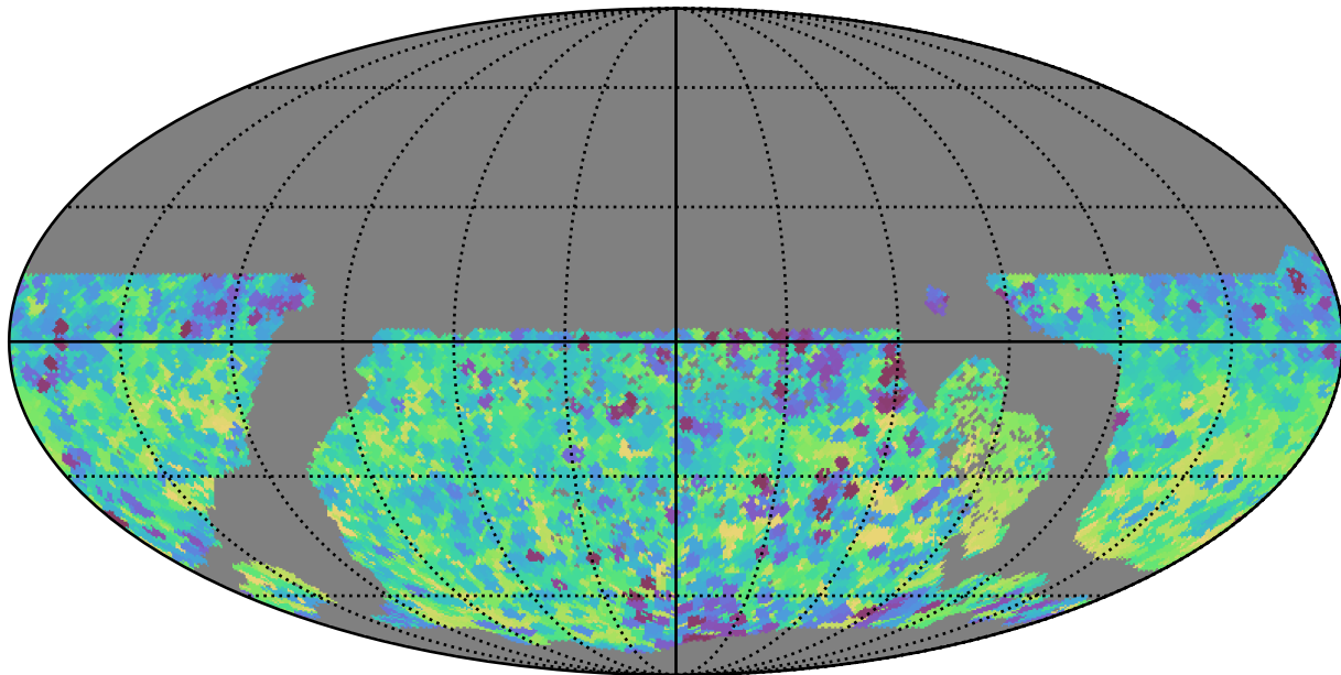
extra_ss_neo7_v3.4_10yrs WFD y band: Min skyBrightness
