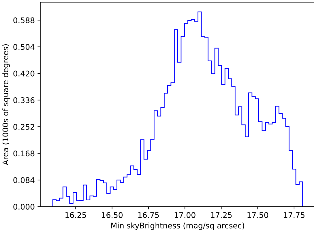
extra_ss_neo7_v3.4_10yrs WFD y band: Min skyBrightness
