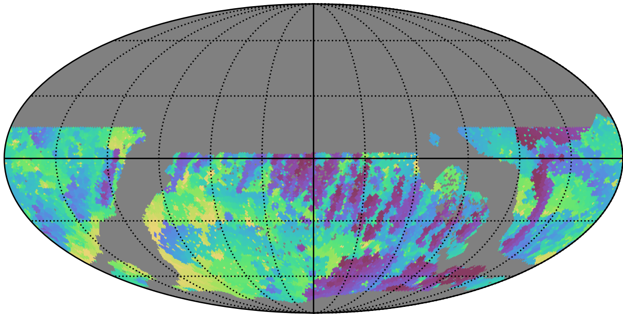
extra_ss_neo7_v3.4_10yrs WFD r band: Min skyBrightness
