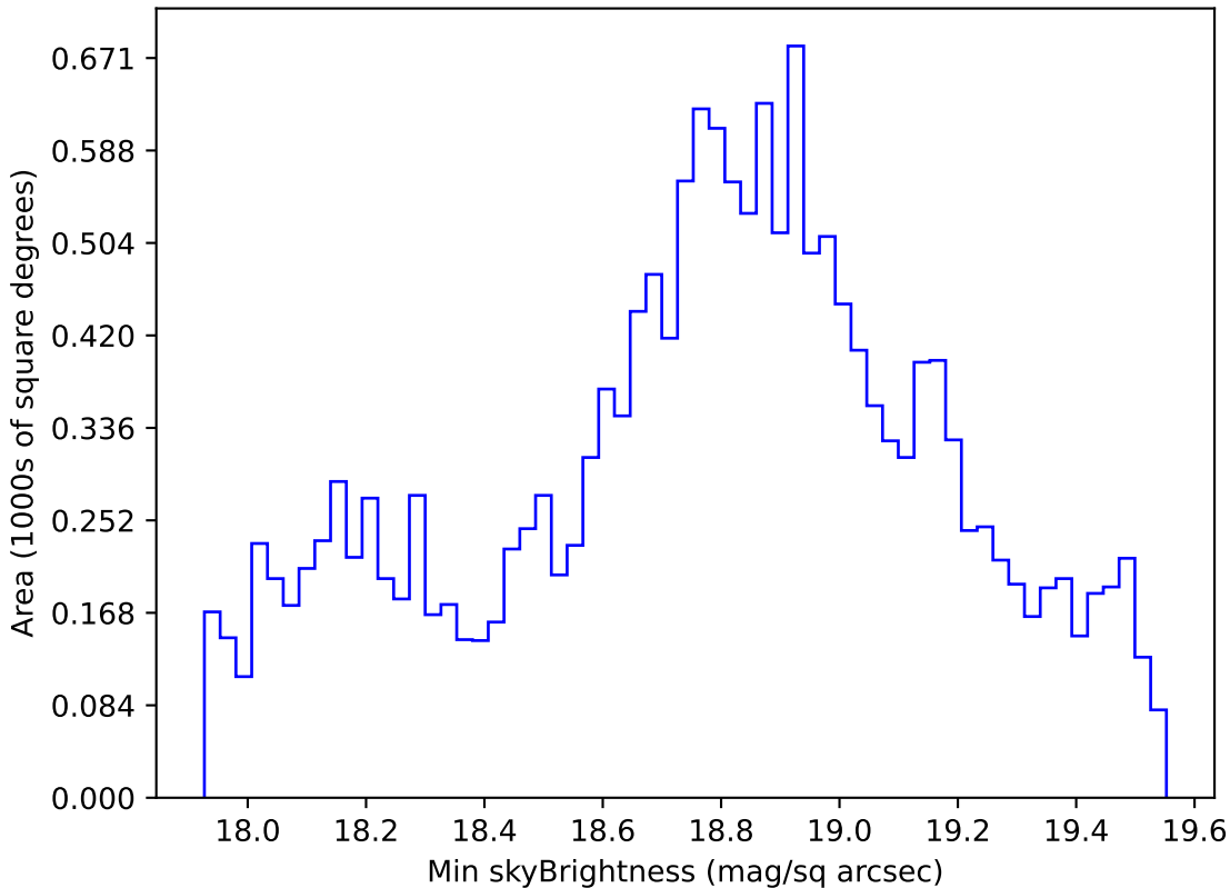
extra_ss_neo7_v3.4_10yrs WFD r band: Min skyBrightness
