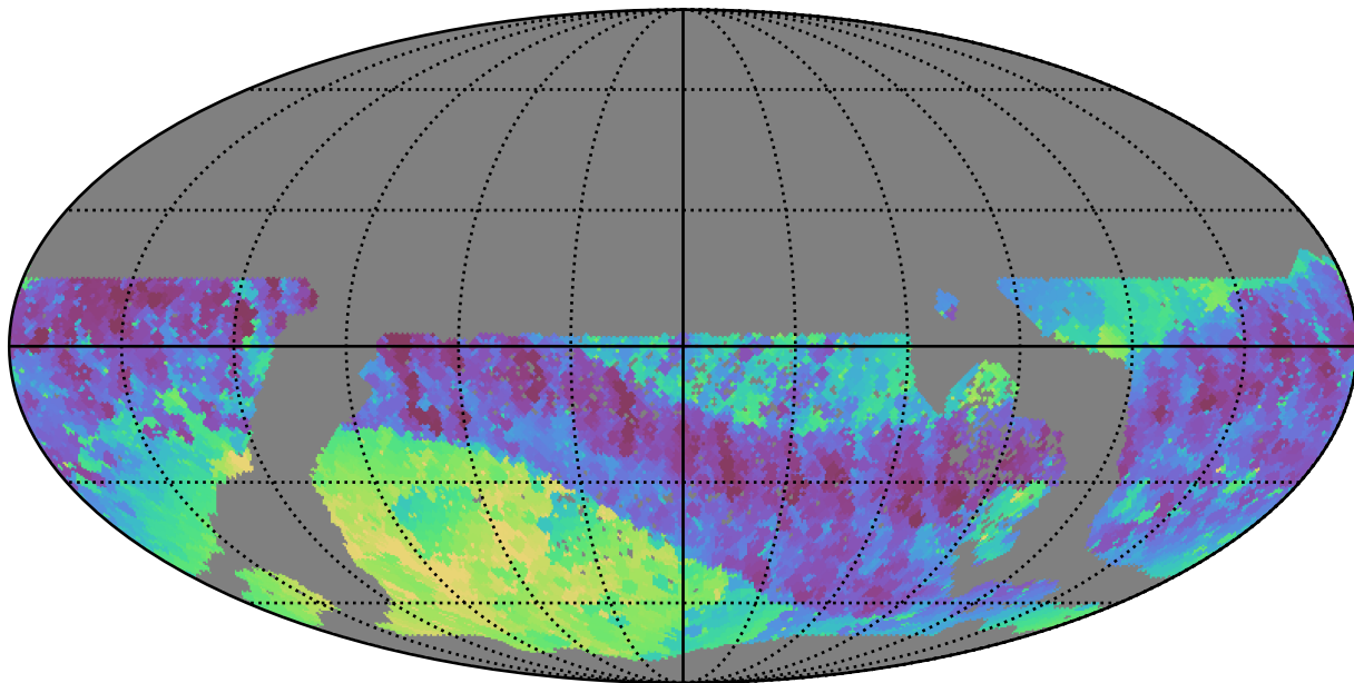
extra_ss_neo7_v3.4_10yrs WFD i band: Min skyBrightness
