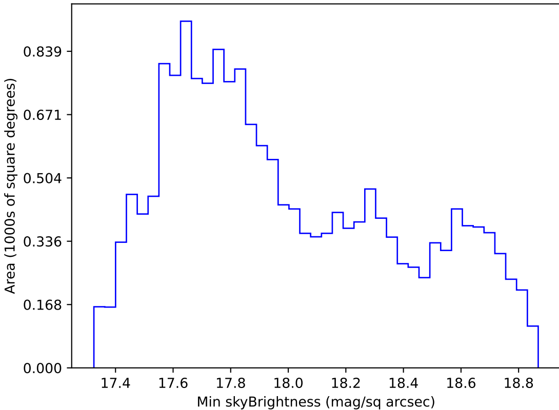
extra_ss_neo7_v3.4_10yrs WFD i band: Min skyBrightness
