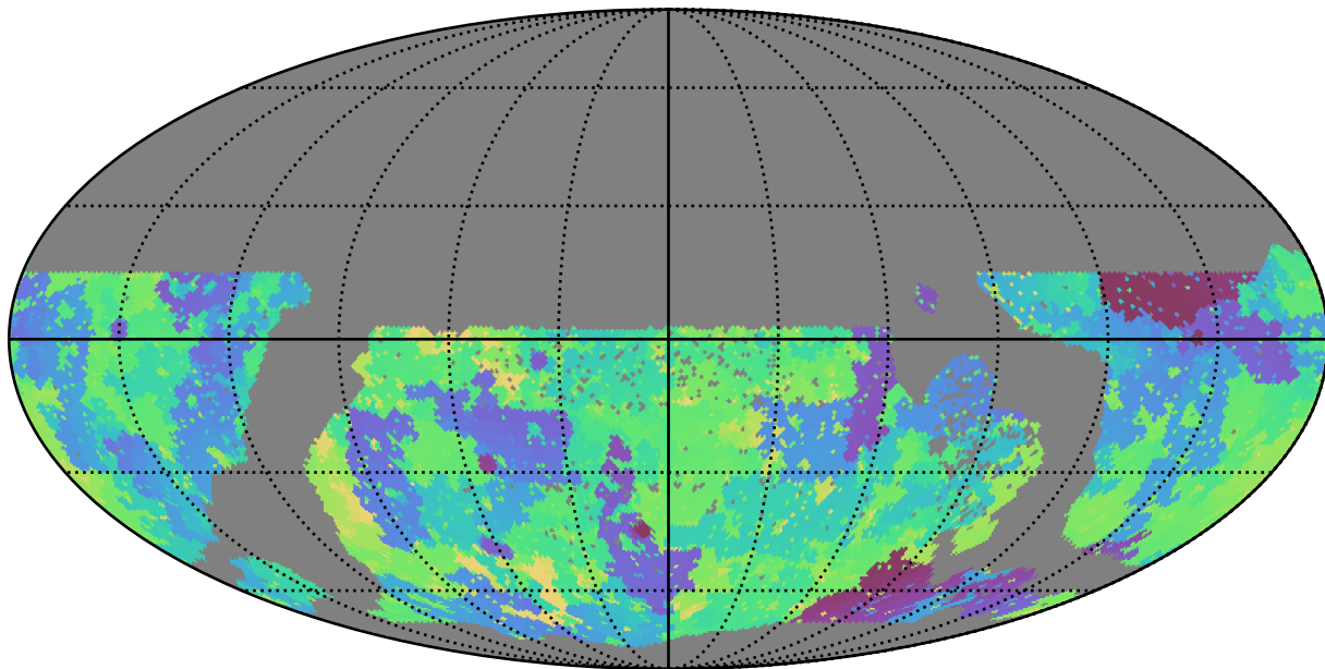
extra_ss_neo7_v3.4_10yrs WFD g band: Min skyBrightness
