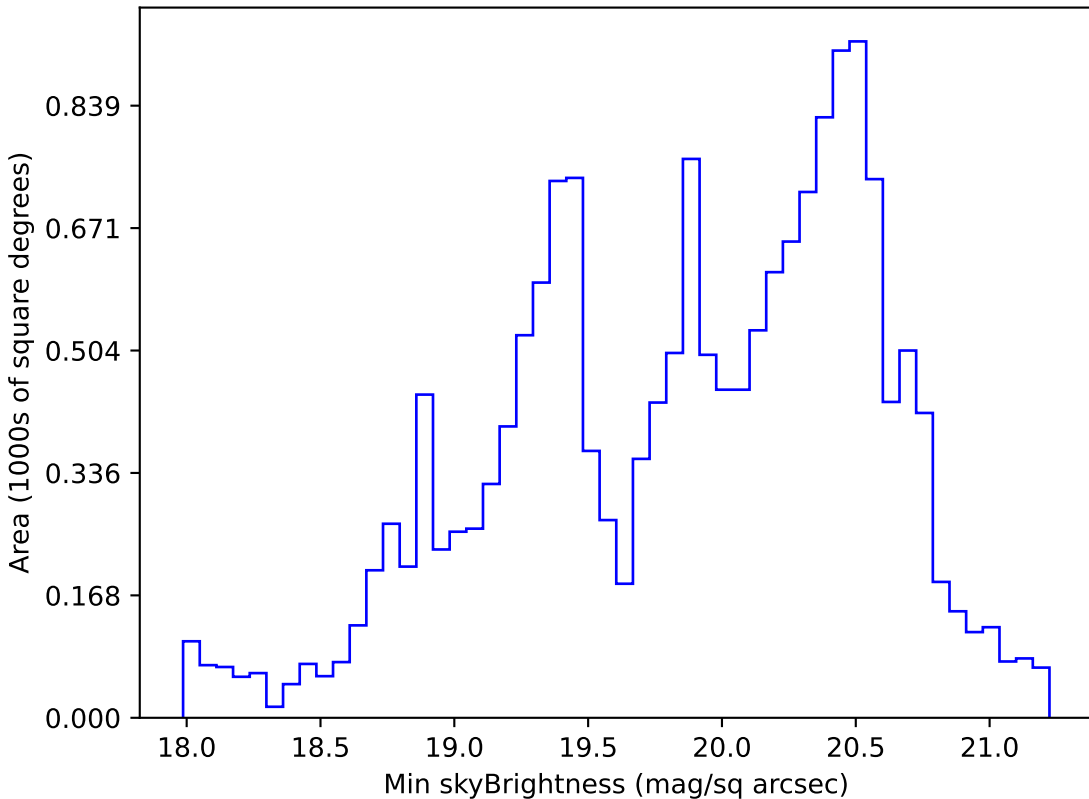
extra_ss_neo7_v3.4_10yrs WFD g band: Min skyBrightness
