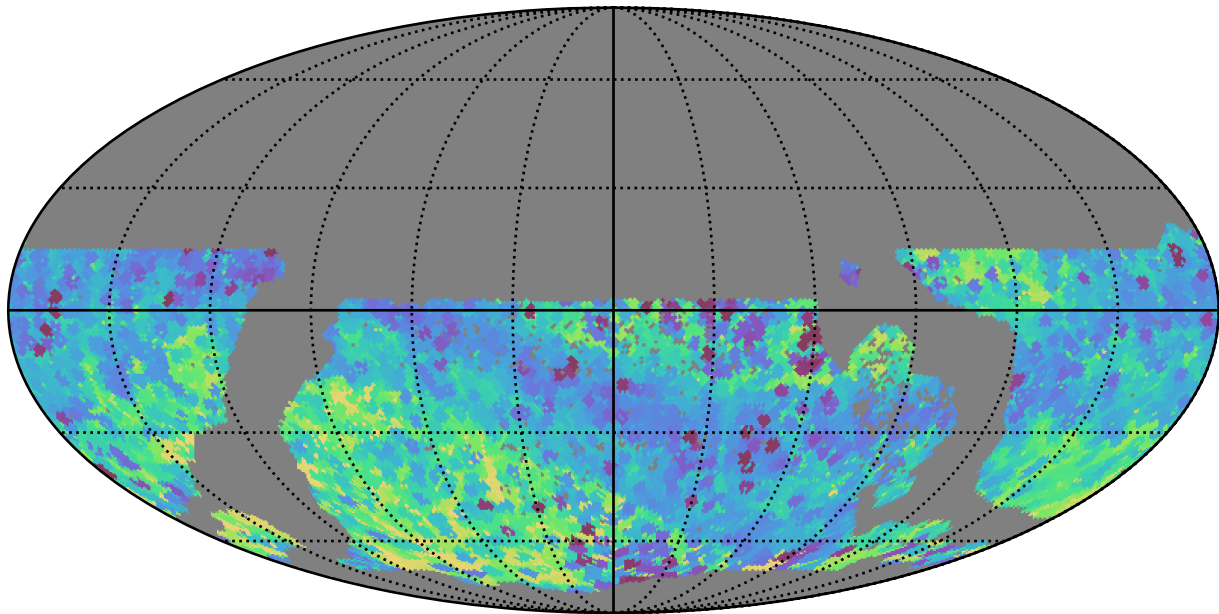
extra_ss_neo7_v3.4_10yrs WFD all bands: Min skyBrightness
