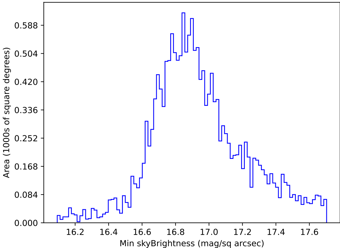
extra_ss_neo7_v3.4_10yrs WFD all bands: Min skyBrightness
