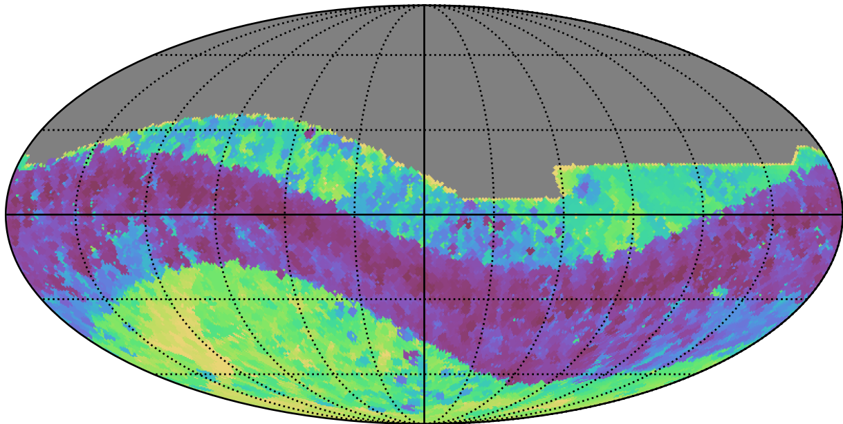
extra_ss_neo7_v3.4_10yrs All sky z band: Min skyBrightness
