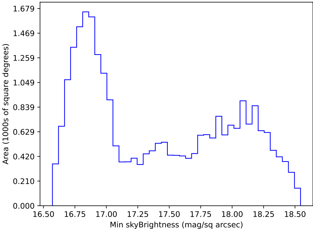
extra_ss_neo7_v3.4_10yrs All sky z band: Min skyBrightness
