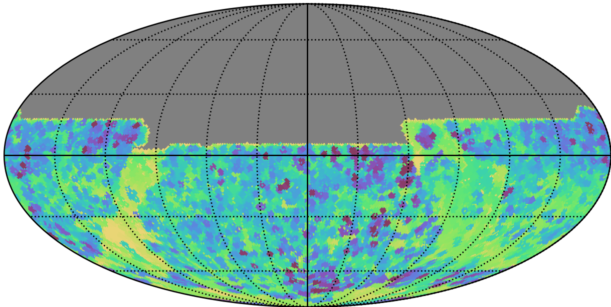
extra_ss_neo7_v3.4_10yrs All sky y band: Min skyBrightness
