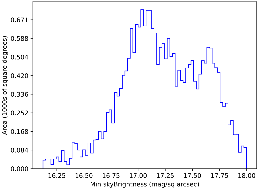
extra_ss_neo7_v3.4_10yrs All sky y band: Min skyBrightness
