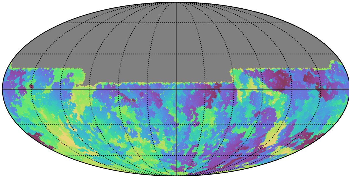
extra_ss_neo7_v3.4_10yrs All sky u band: Min skyBrightness
