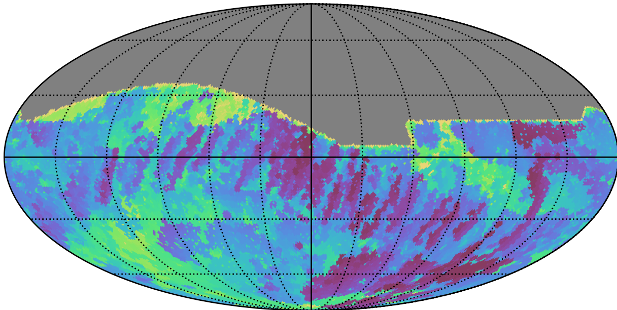
extra_ss_neo7_v3.4_10yrs All sky r band: Min skyBrightness
