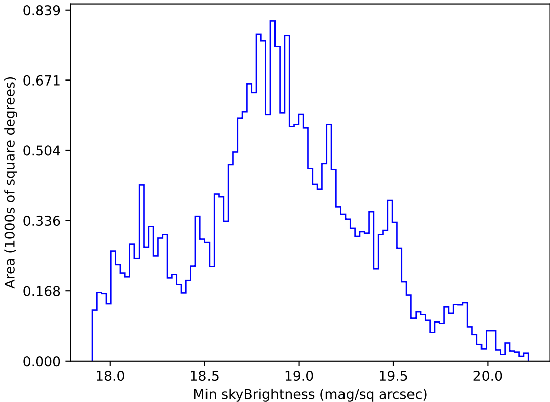
extra_ss_neo7_v3.4_10yrs All sky r band: Min skyBrightness
