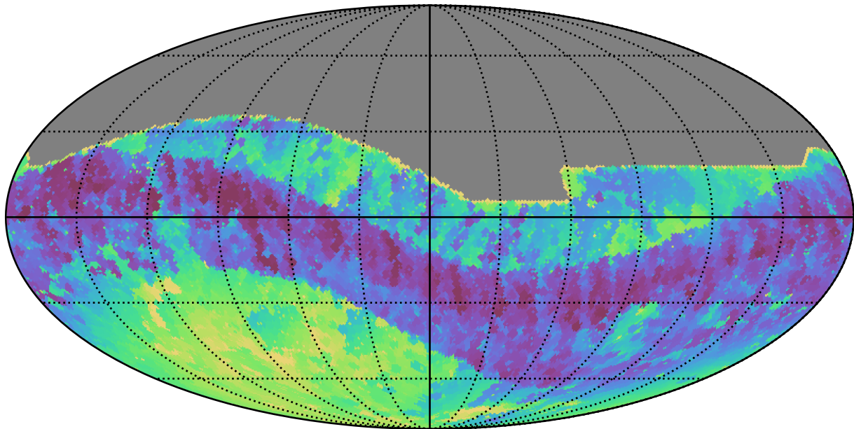
extra_ss_neo7_v3.4_10yrs All sky i band: Min skyBrightness
