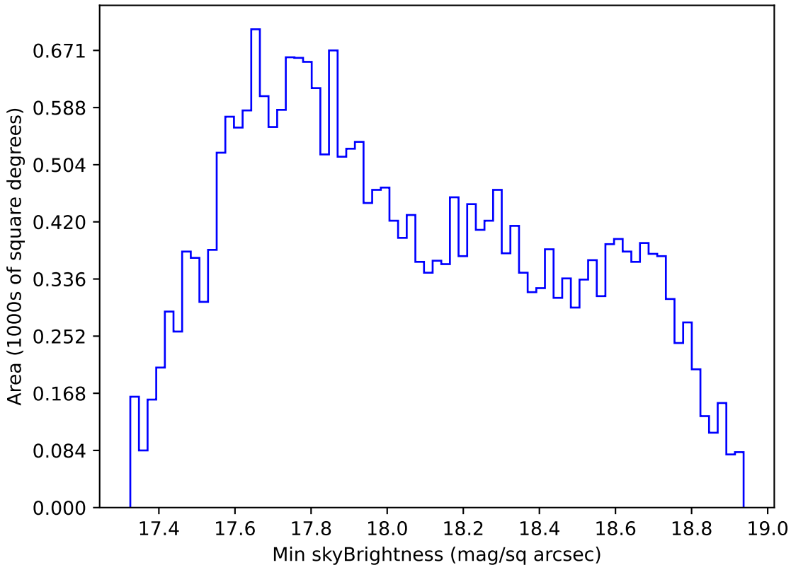
extra_ss_neo7_v3.4_10yrs All sky i band: Min skyBrightness
