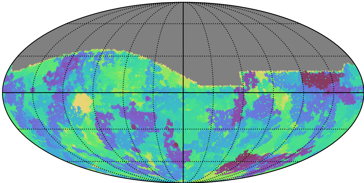
extra_ss_neo7_v3.4_10yrs All sky g band: Min skyBrightness
