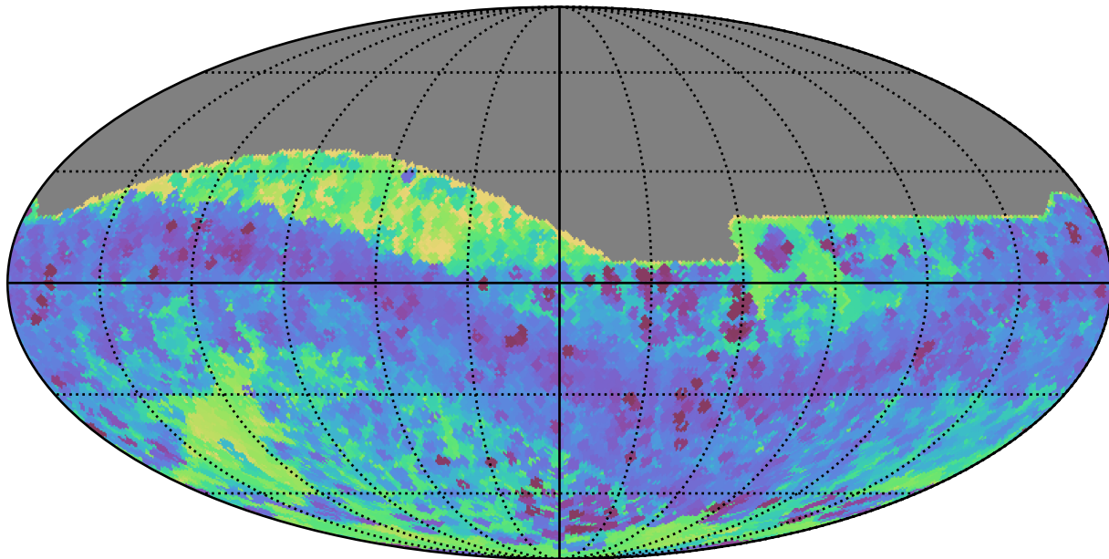
extra_ss_neo7_v3.4_10yrs All sky all bands: Min skyBrightness
