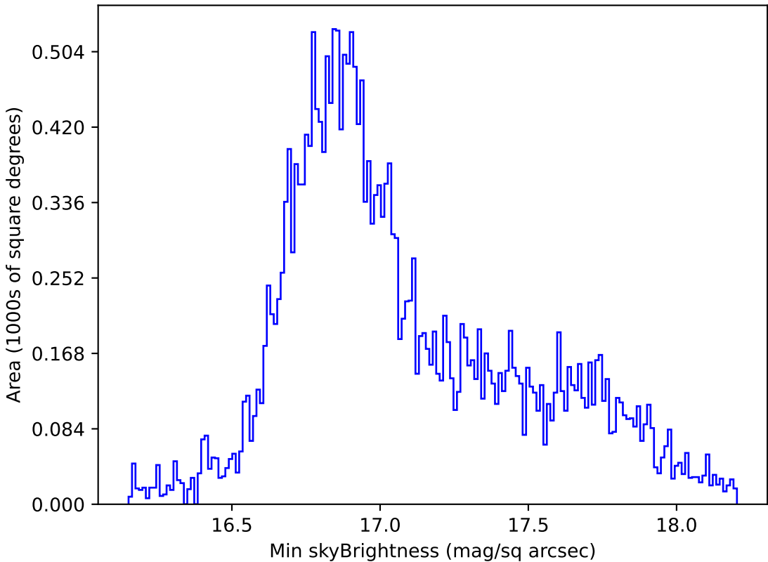
extra_ss_neo7_v3.4_10yrs All sky all bands: Min skyBrightness
