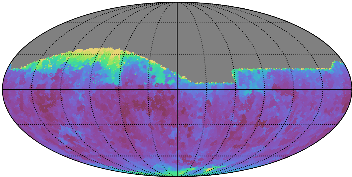
extra_ss_neo7_v3.4_10yrs Yr 1 all bands: Min seeingGeom
