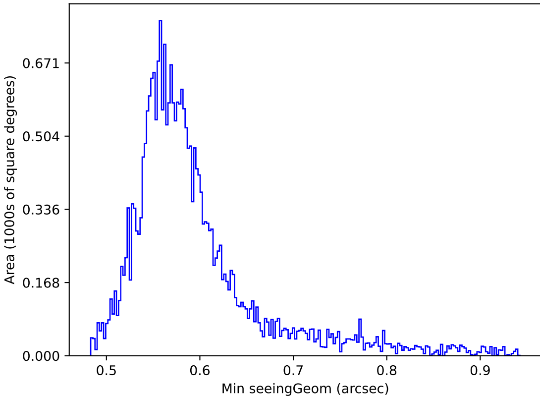
extra_ss_neo7_v3.4_10yrs Yr 1 all bands: Min seeingGeom
