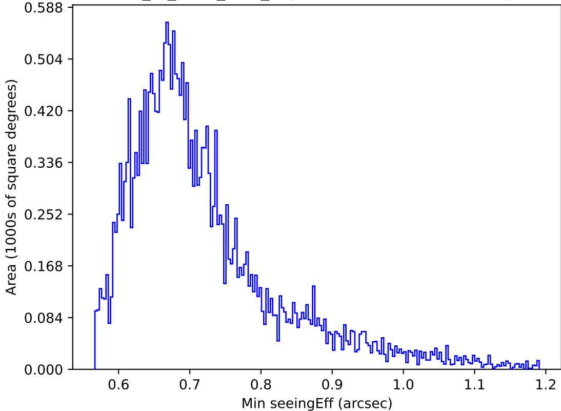
extra_ss_neo7_v3.4_10yrs Yr 1 z band: Min seeingEff
