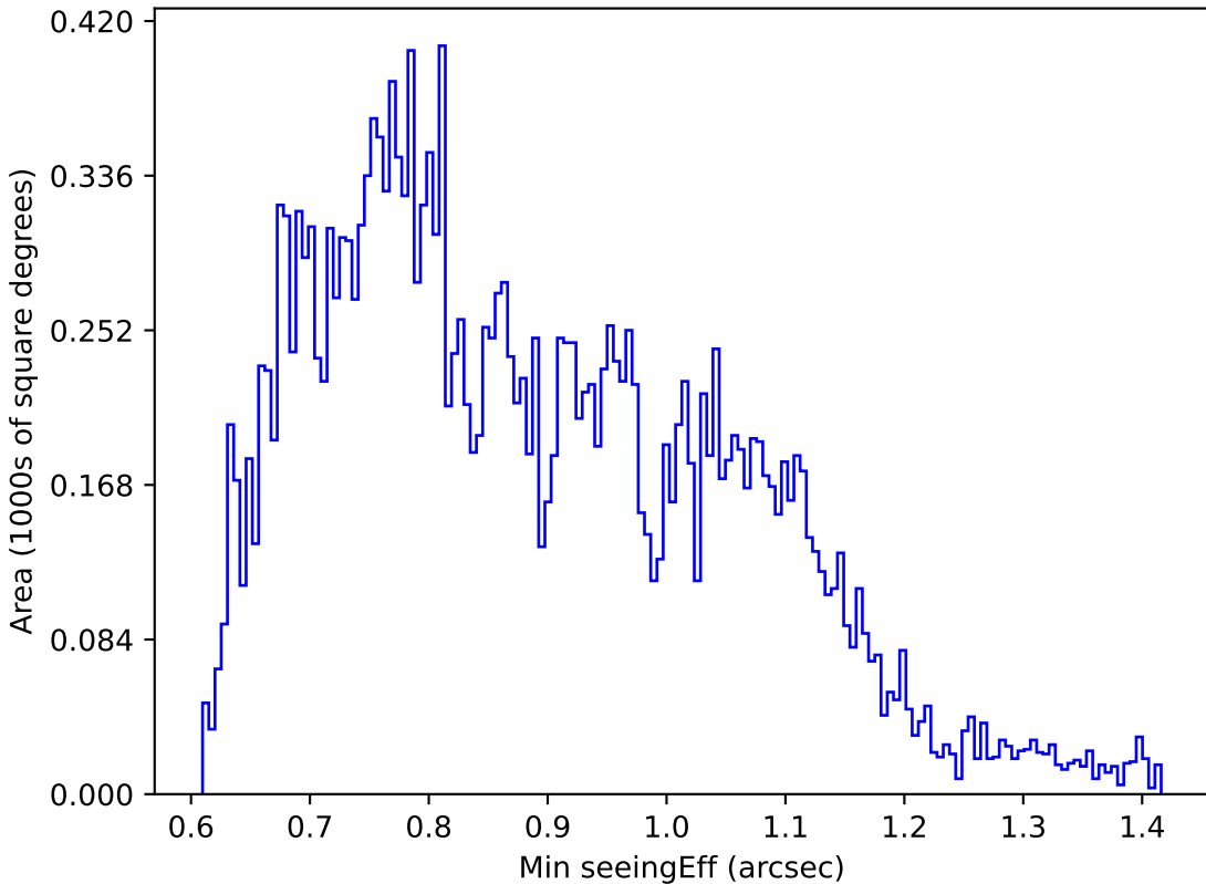
extra_ss_neo7_v3.4_10yrs Yr 1 u band: Min seeingEff
