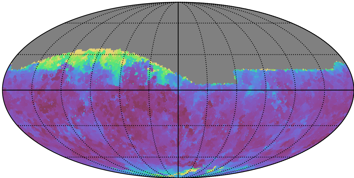
extra_ss_neo7_v3.4_10yrs Yr 1 r band: Min seeingEff
