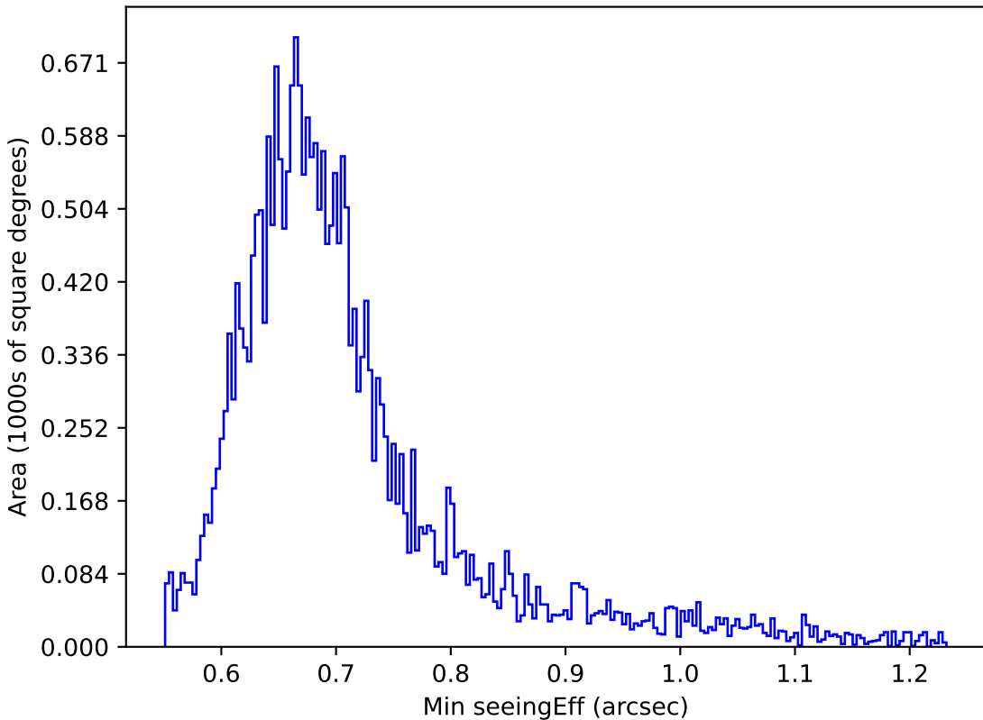
extra_ss_neo7_v3.4_10yrs Yr 1 i band: Min seeingEff
