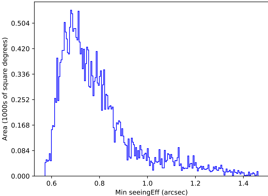
extra_ss_neo7_v3.4_10yrs Yr 1 g band: Min seeingEff
