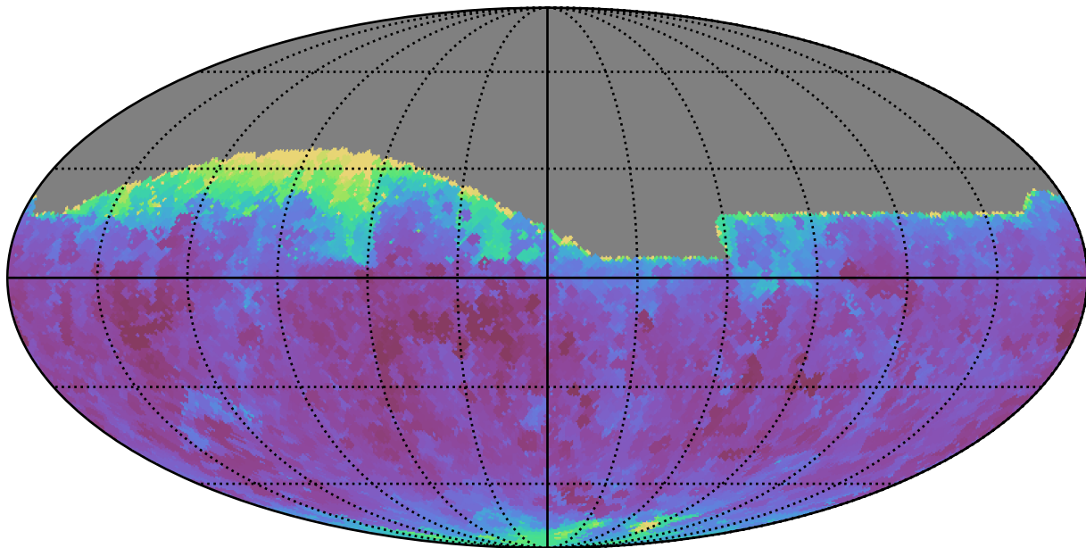
extra_ss_neo7_v3.4_10yrs Yr 1 all bands: Min seeingEff
