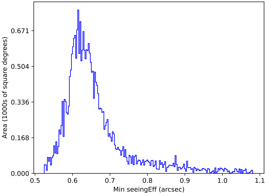
extra_ss_neo7_v3.4_10yrs Yr 1 all bands: Min seeingEff
