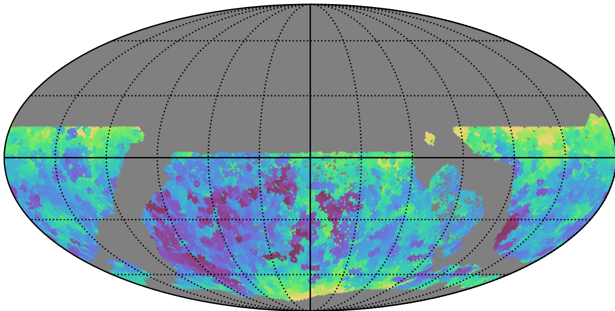
extra_ss_neo7_v3.4_10yrs WFD z band: Min seeingEff
