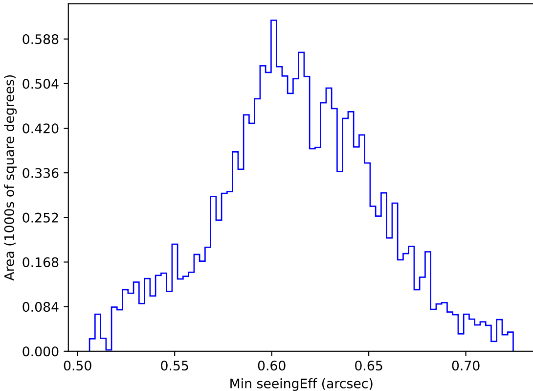
extra_ss_neo7_v3.4_10yrs WFD z band: Min seeingEff
