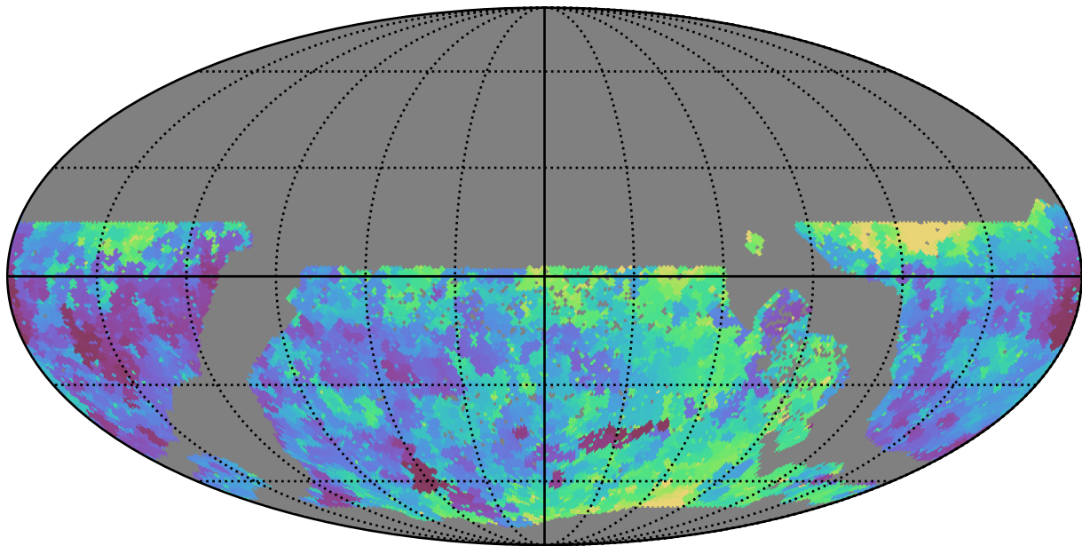
extra_ss_neo7_v3.4_10yrs WFD u band: Min seeingEff
