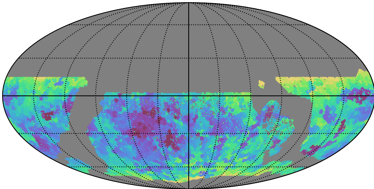
extra_ss_neo7_v3.4_10yrs WFD r band: Min seeingEff
