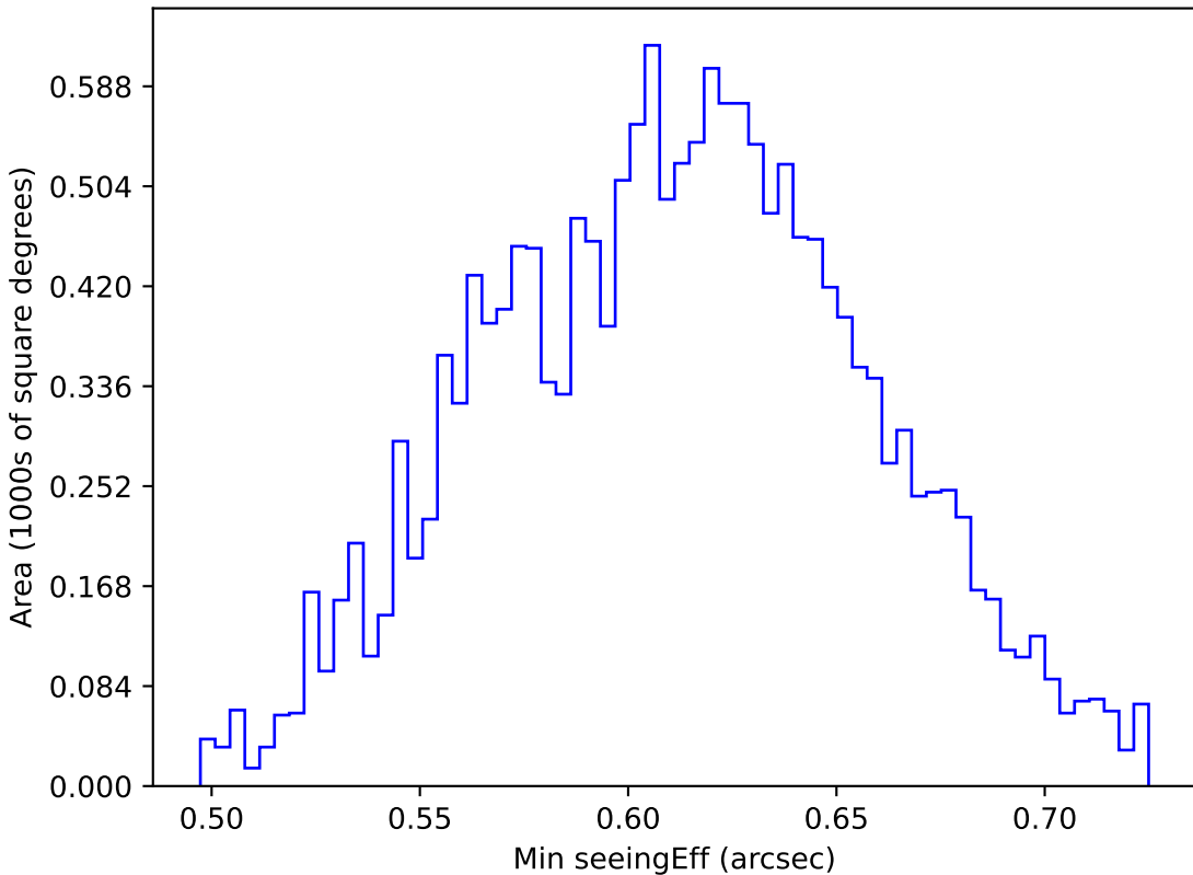
extra_ss_neo7_v3.4_10yrs WFD r band: Min seeingEff
