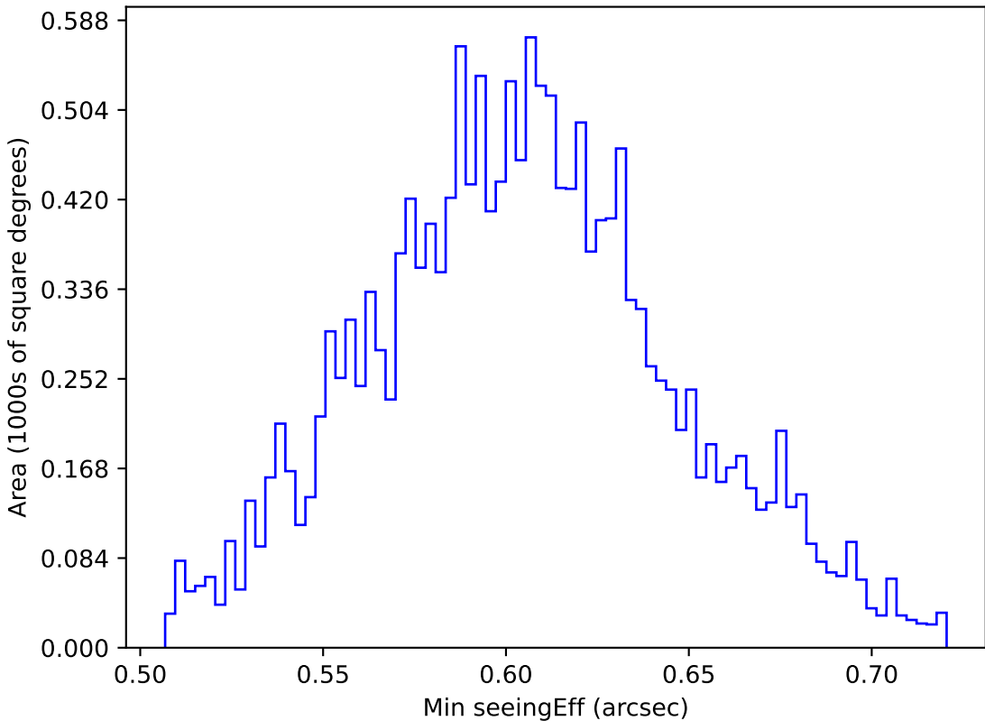
extra_ss_neo7_v3.4_10yrs WFD i band: Min seeingEff
